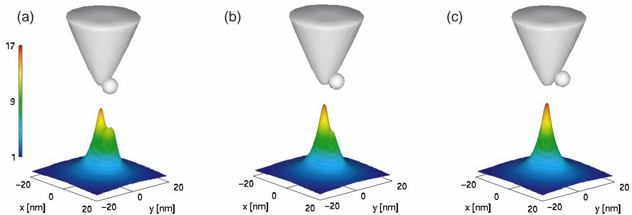
Fig. 5. Relative electric field intensity distribution 2 nm below a tungsten tip with a \rho \approx 8 nm protrusion located at different altitudes z relative to the apex: (a) z = -2 nm; (b) z = 0 and (c) z = 2 nm.
